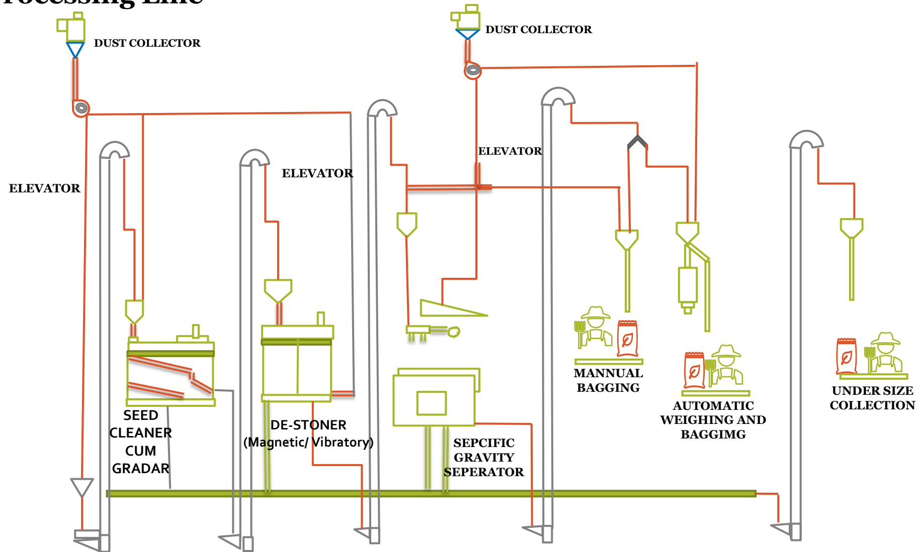
LAYOUT OF GRAIN PROCESSING PLANT
